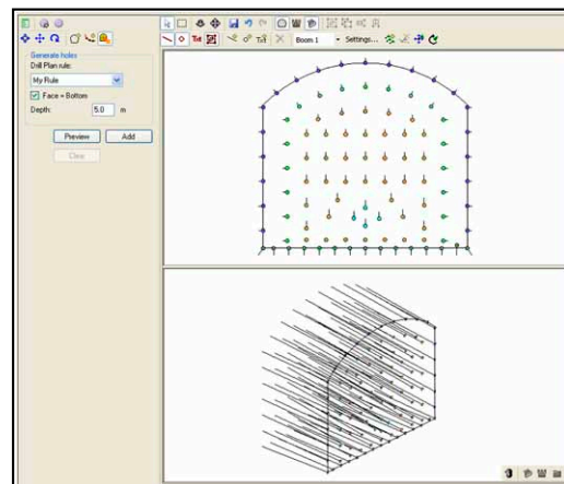
Drill plan generated in Drill Plan Generator.
