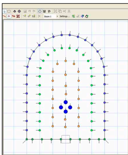
Drill plan designed in Tunnel Manager.
