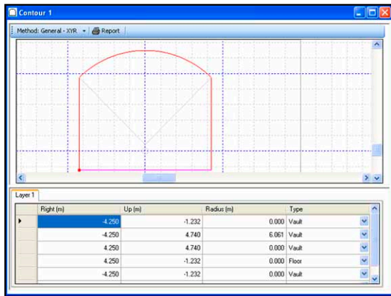
Contour of a tunnel.
