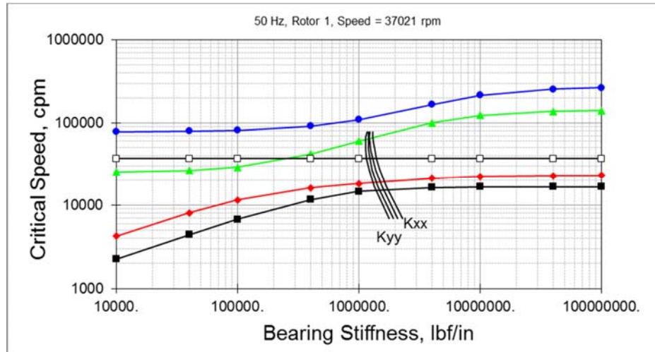
Figure 4: Critical speed map.
