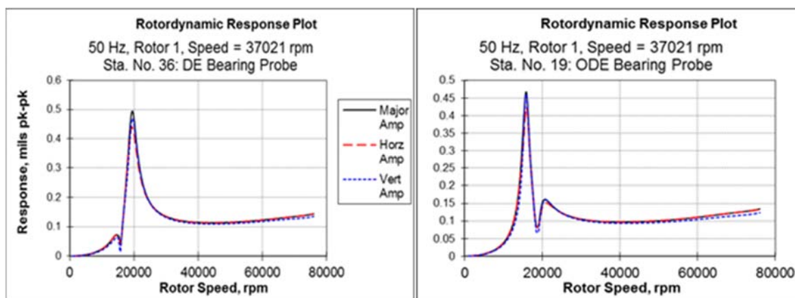
Figure 5: Unbalance response.
