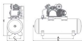
AT2/AT3/AT5/AT7
