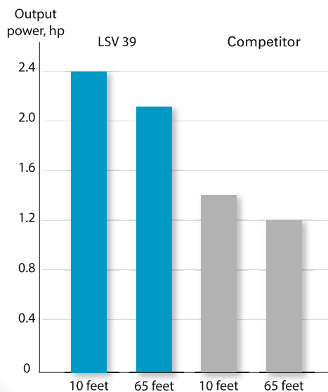
Power at different hose lengths 5" angle grinder.
