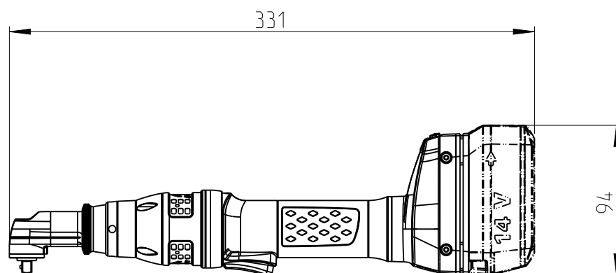
14V Battery
