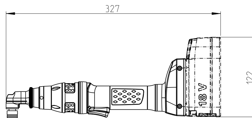
18V Battery
